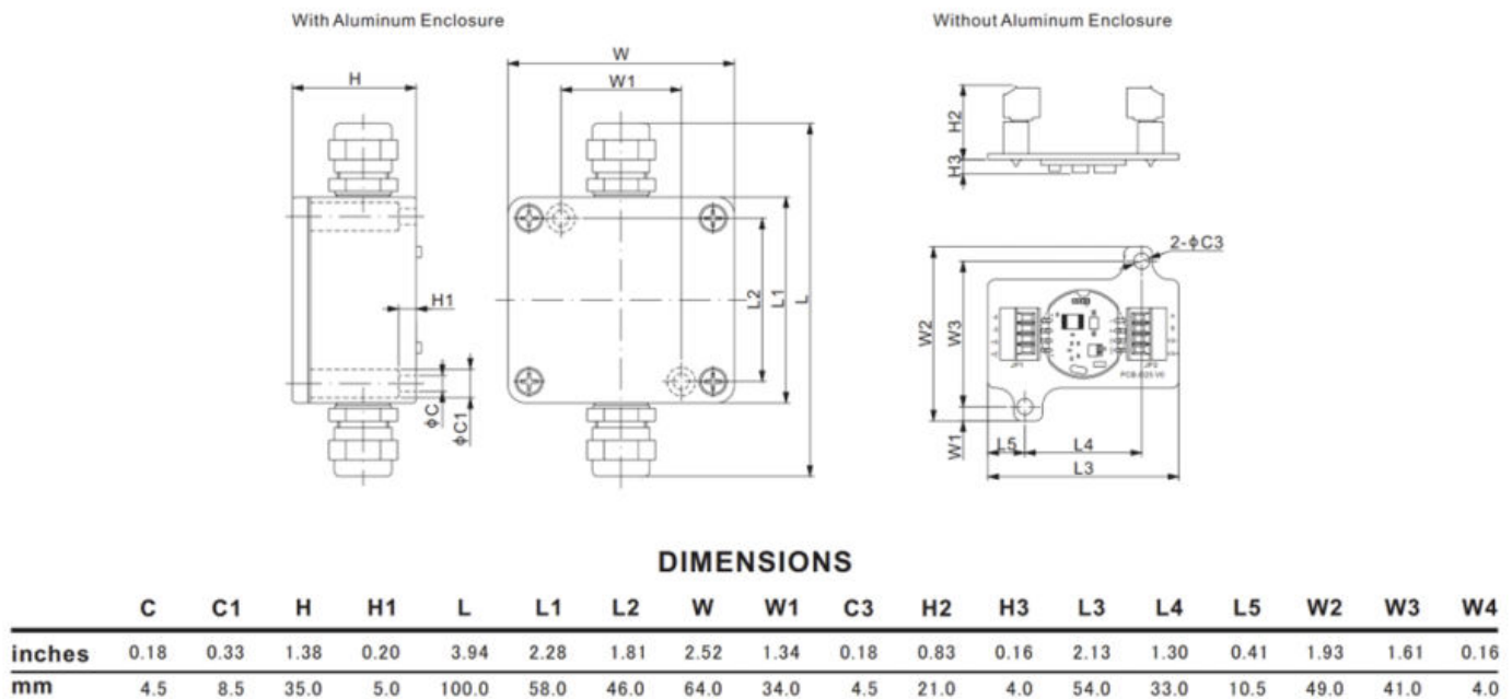
Figure 7-1. Chip Dimensions (With and Without Enclosure)
