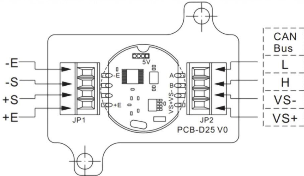
Figure 2-1: Connection Diagram for DGB-DC2508C
